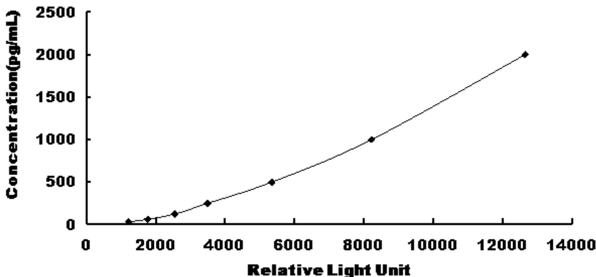
Typical Standard Curve for Mouse IFNg CLIA.
